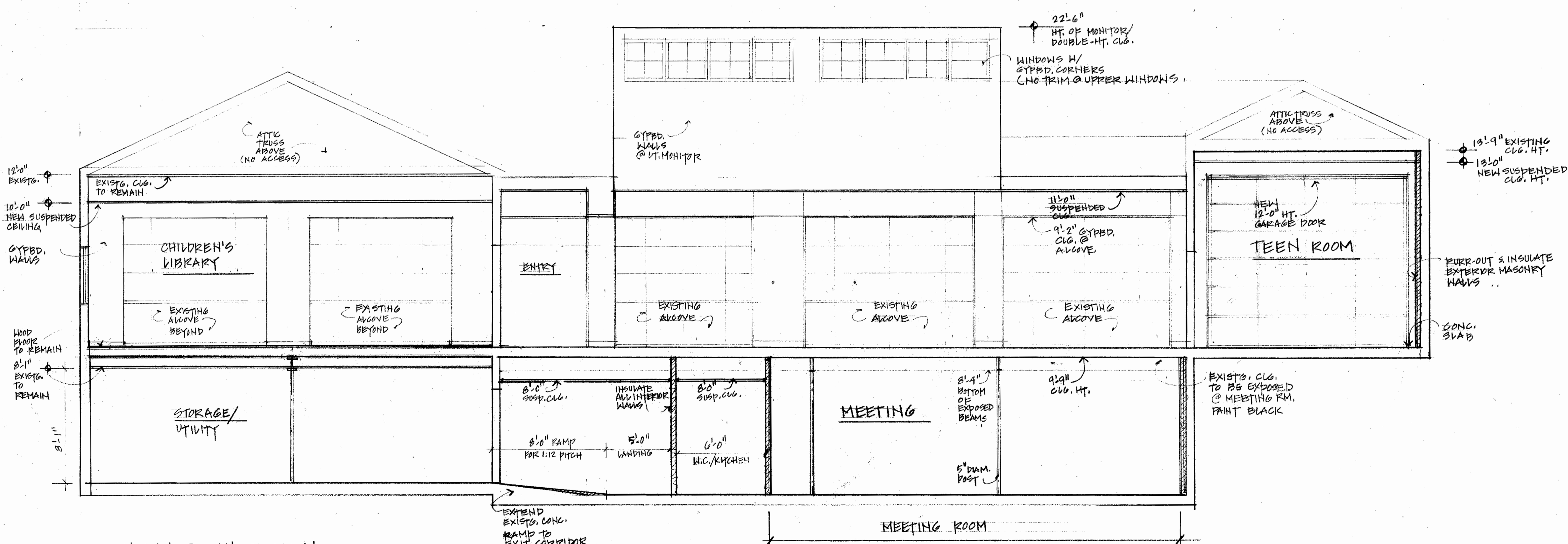
2 NORTH-SOUTH SECTION 1/4" = 1'-0"
